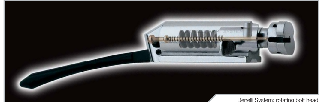
Benelli System: rotating bolt head
