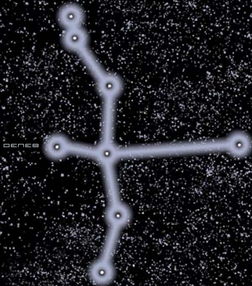
CYGNUS, the Swan Constellation
