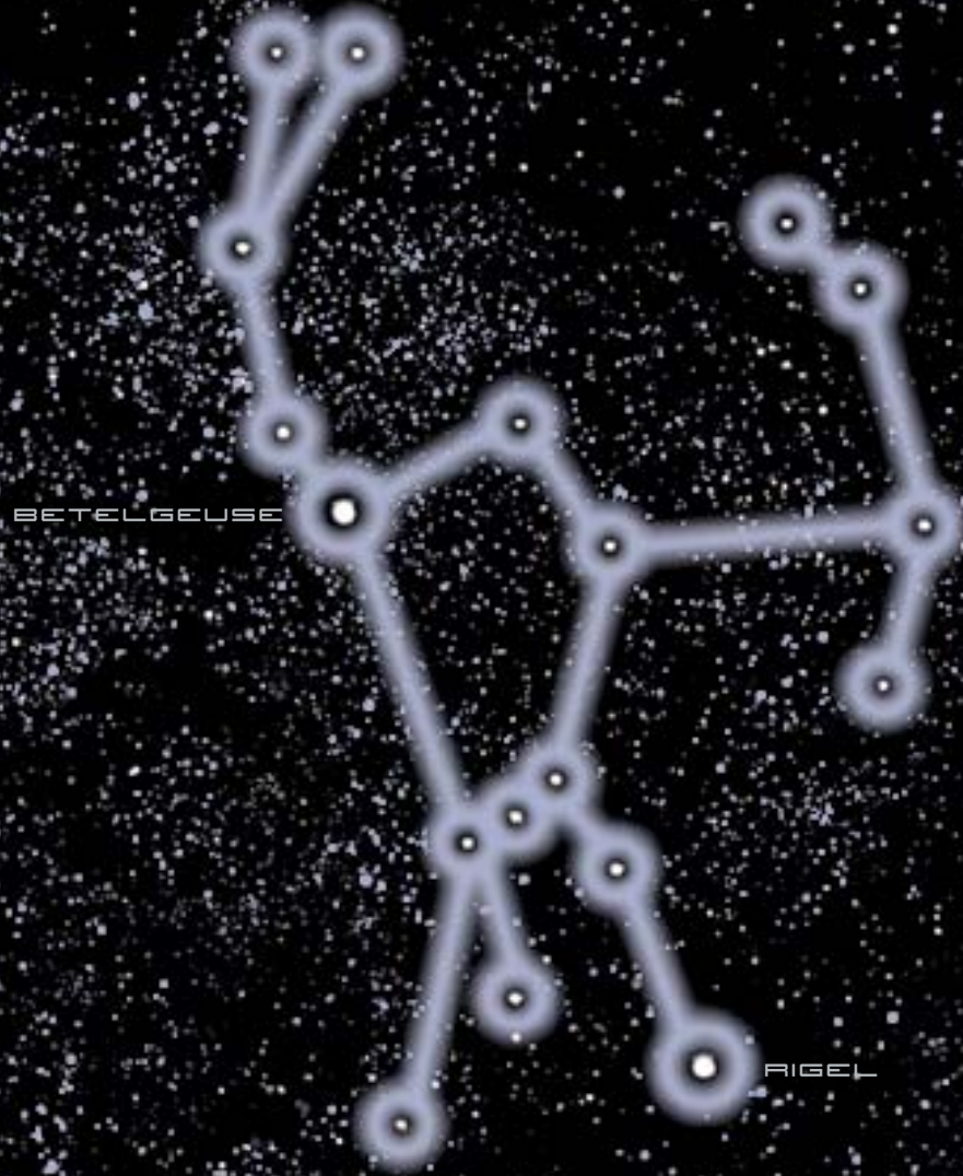
The ORION Constellation
